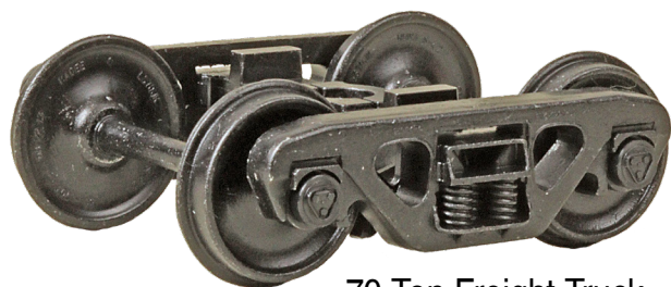
70-Ton Freight Truck Bearing caps rotate
